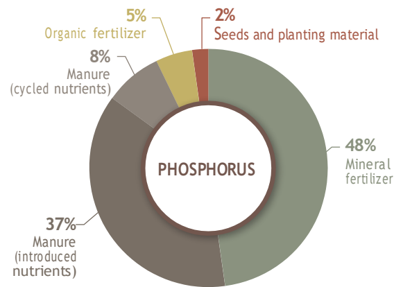
Figure 8: Sources of phosphorus flowing into crop production.
